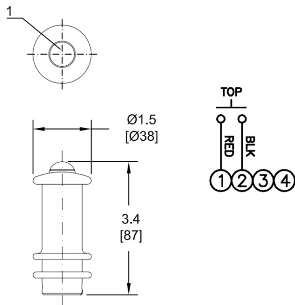
MG9 dimensions & wiring details
