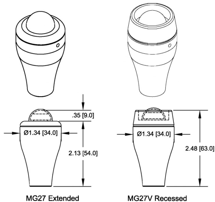
MG27 extended & recessed dimensions
