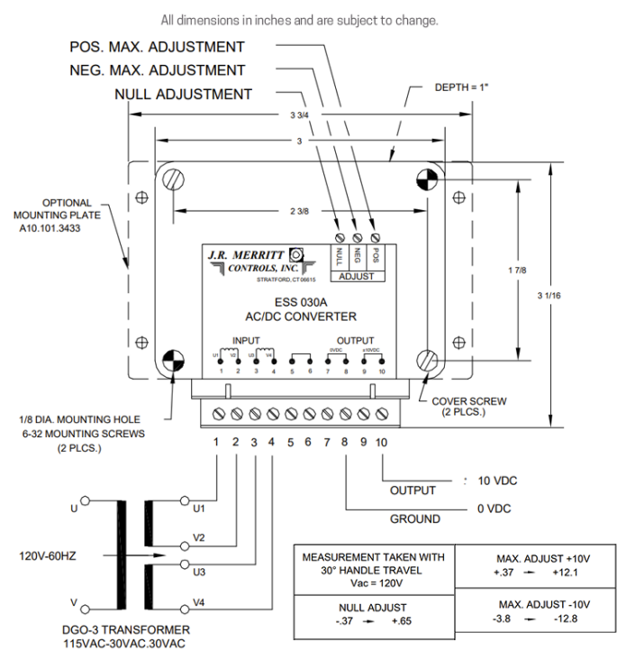
ESS 03A dimensions and wiring details
