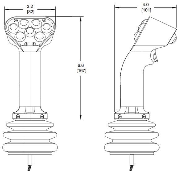
FG5 dimensions
